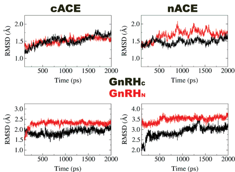
FIGURE 3: Root-mean-square deviation as a function of simulation time from the initial model of ACE Cα atoms (upper plots) and GnRH all atoms (lower plots) in the complex of cACE (left) or nACE (right) with GnRH C (black lines) or GnRH N (red lines).
